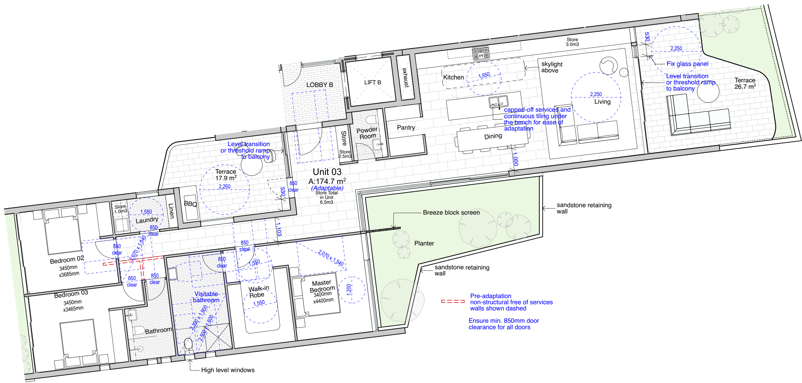
Adaptable unit- Post-adaptation layout
