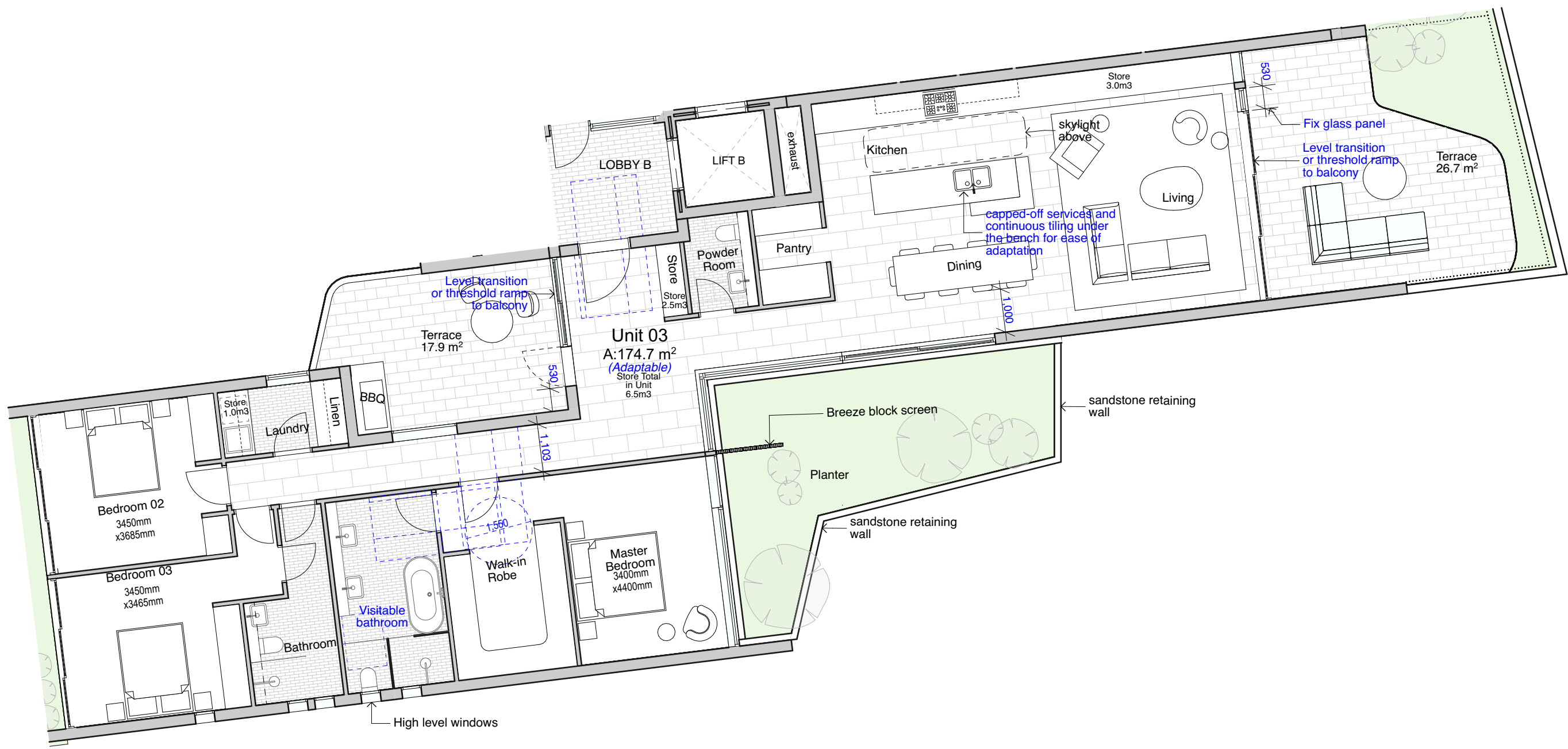
Adaptable unit- Pre-adaptation layout
